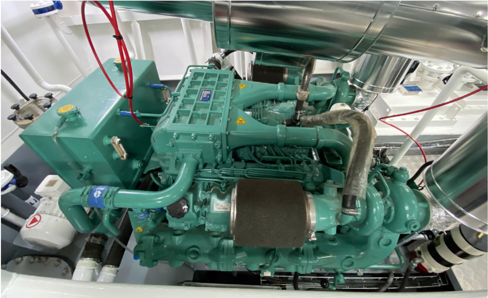
Engine
